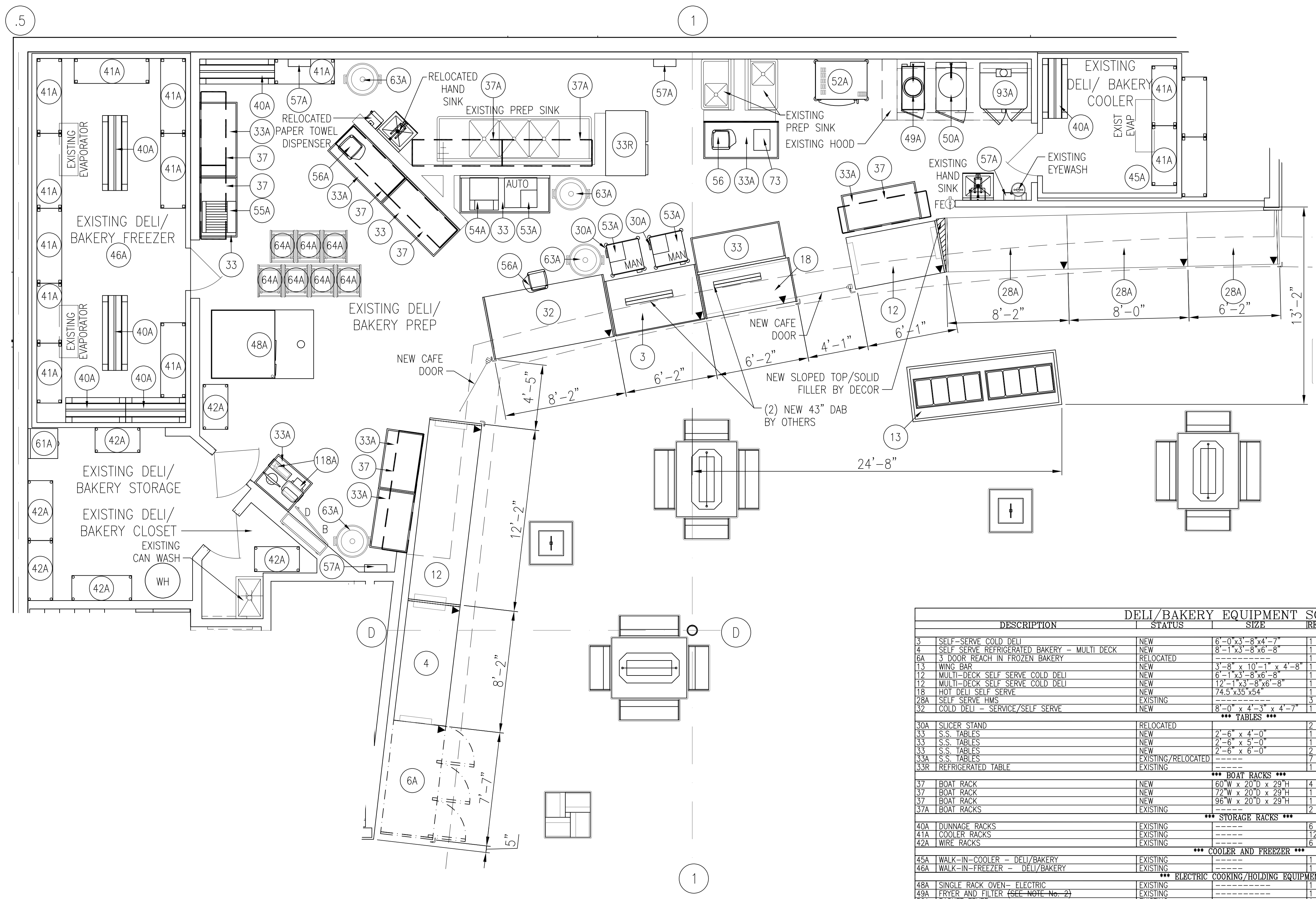
1 DELI/BAKERY FIXTURE PLAN A4.01 1/4" = 1'-0"
