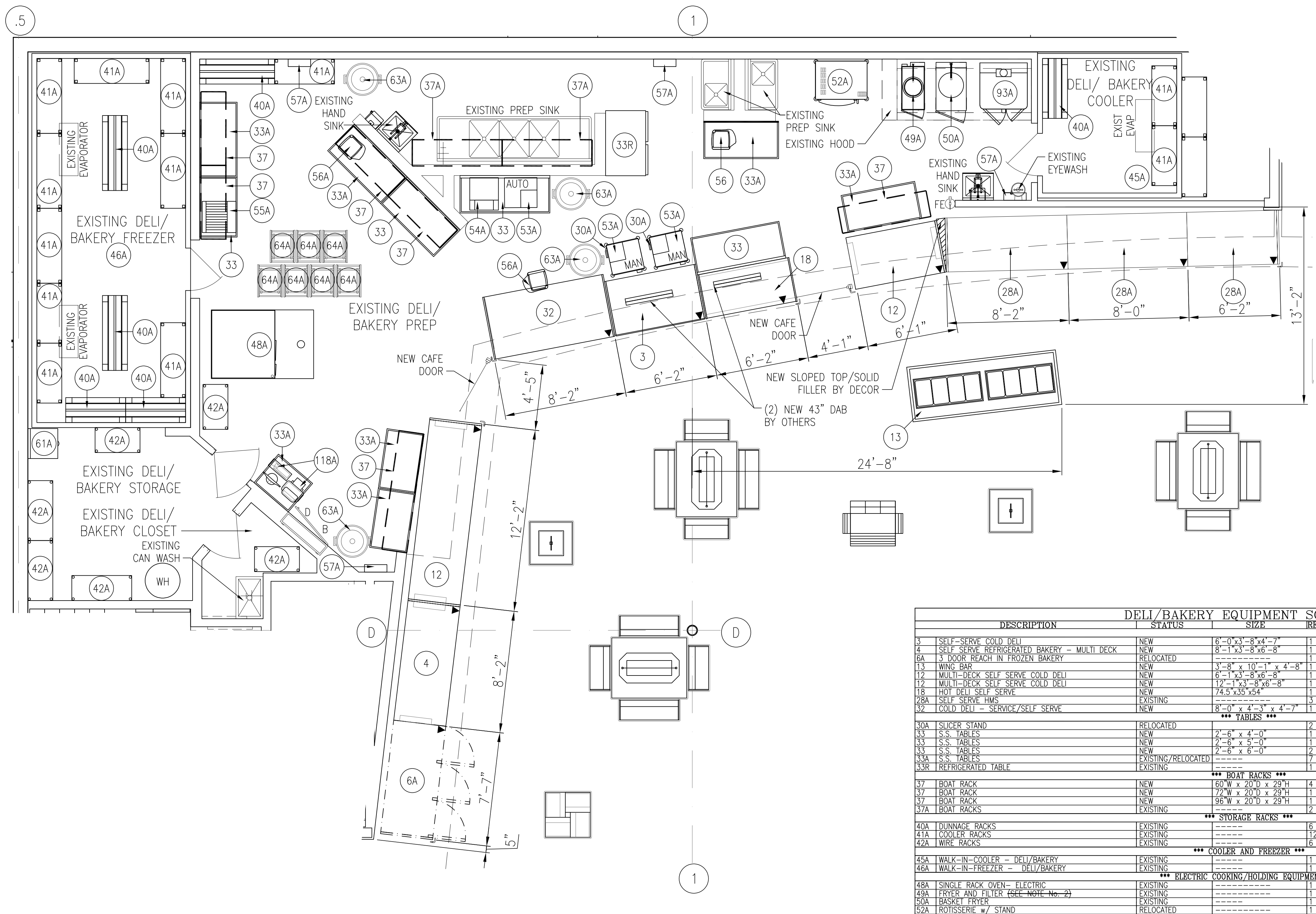
1 DELI/BAKERY FIXTURE PLAN A4.01 1/4" = 1'-0"
