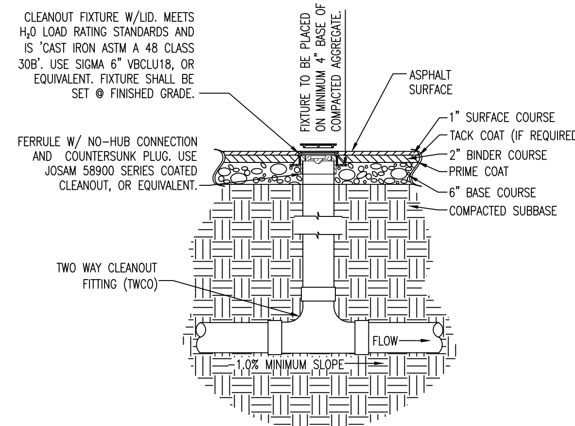
7 TWO-WAY CLEAN OUT SECTION IN ASPHALT P5.01 NTS
