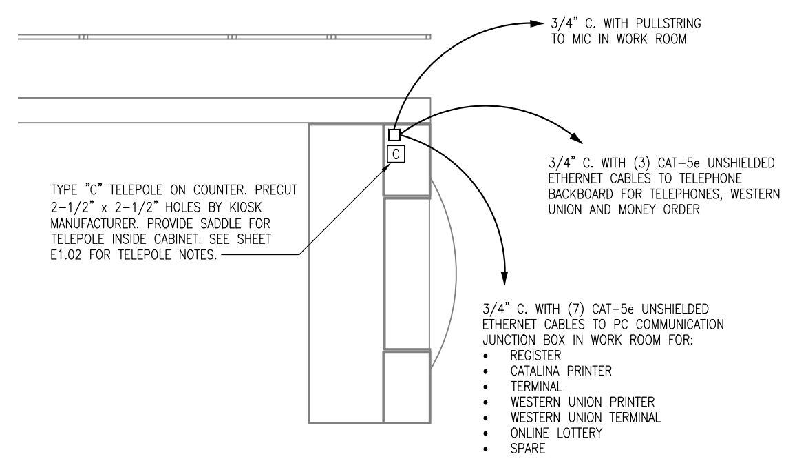
2 CUSTOMER SERVICE KIOSK E4.03 SCALE: 3/8" = 1'-0"
