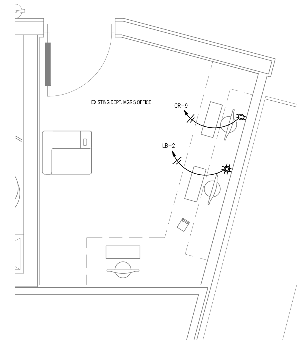
1 DEPARTMENT MANAGERS OFFICE PLAN E4.04 / SCALE: 3/8" = 1'-0"
