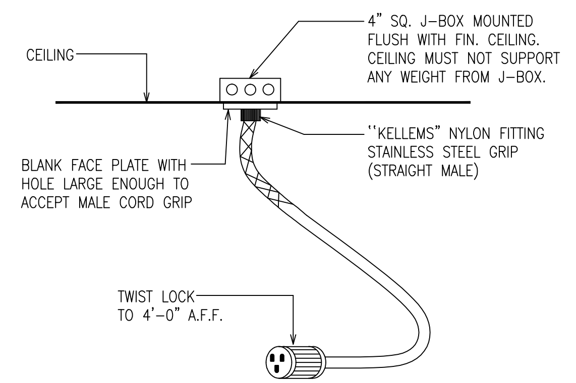
2 HANGING TWIST LOCK DETAIL E5.01 NOT TO SCALE
