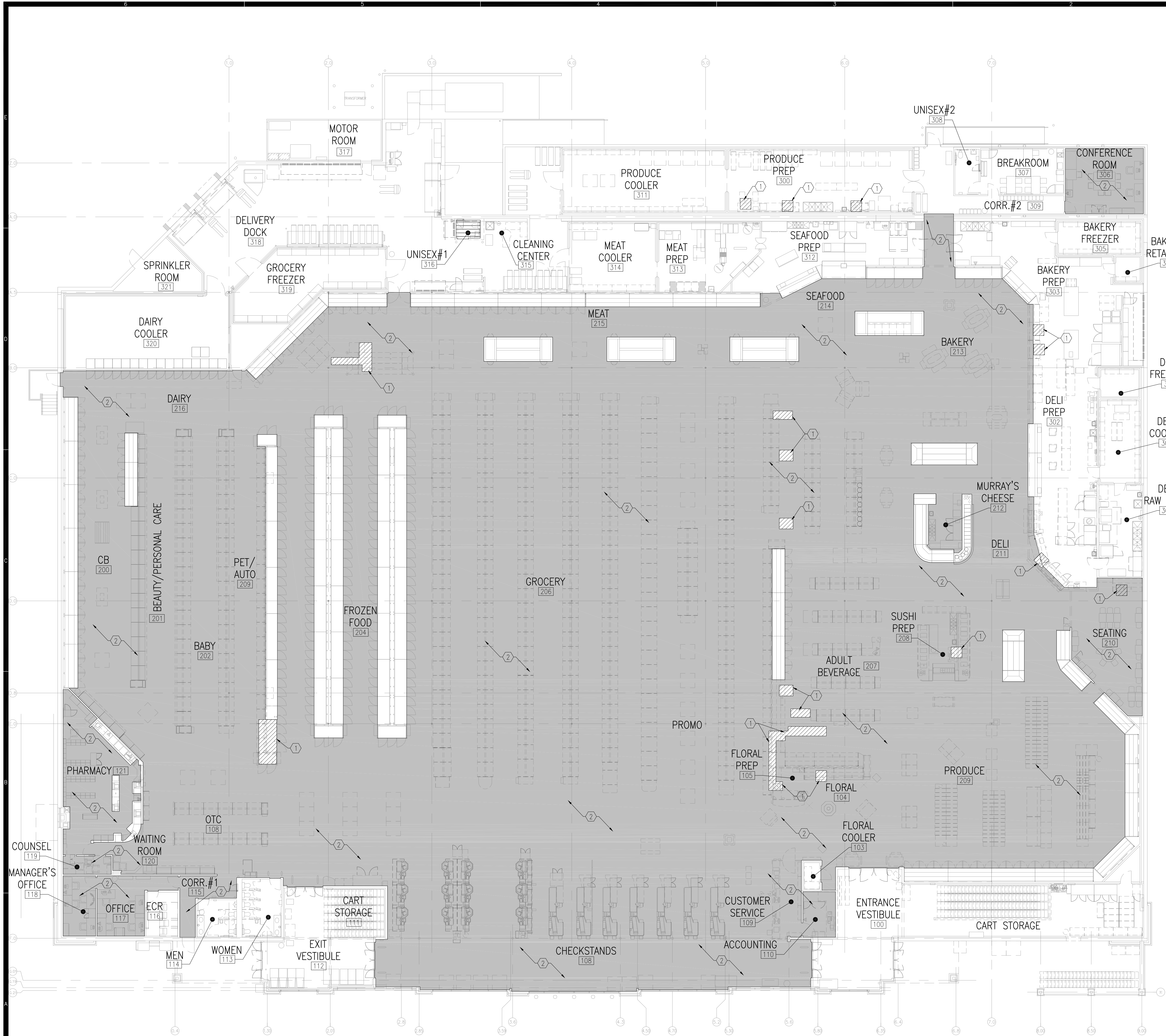
4A DEMOLITION SLAB AND FLOOR FINISHES PLAN SCALE: 3/32" = 1'-0"
