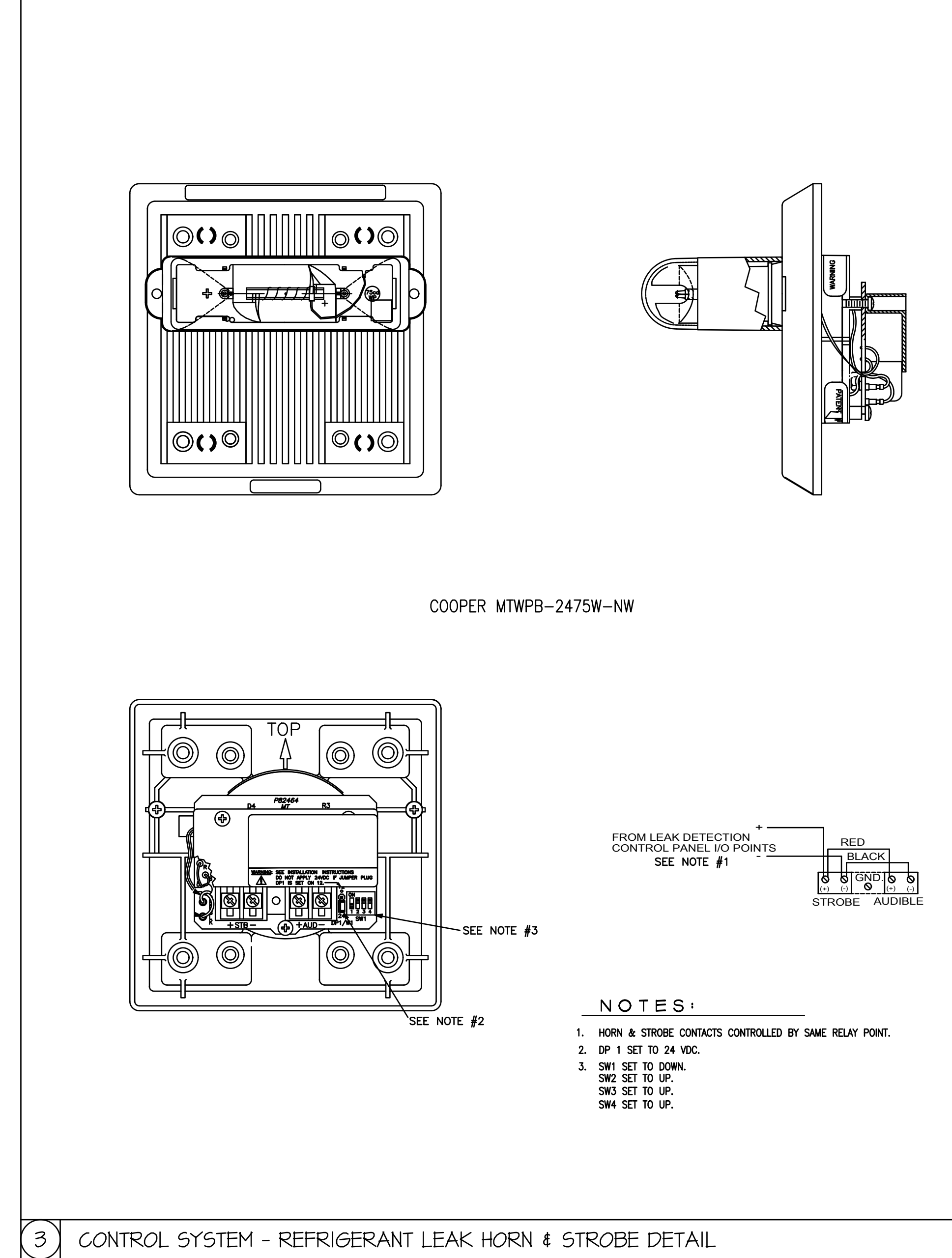
3 CONTROL SYSTEM - REFRIGERANT LEAK HORN & STROBE DETAIL
