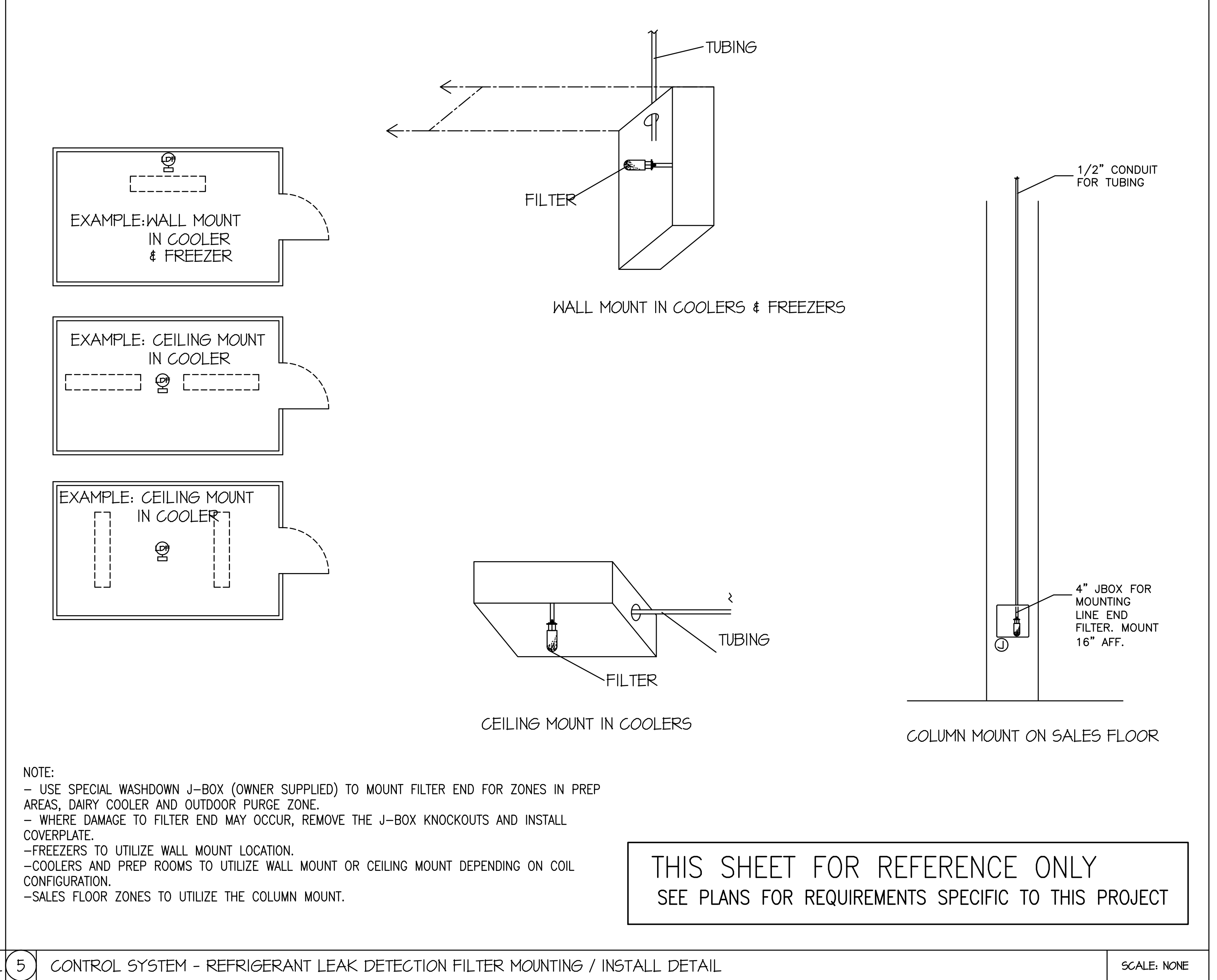
5 CONTROL SYSTEM - REFRIGERANT LEAK DETECTION FILTER MOUNTING / INSTALL DETAIL SCALE: NONE
