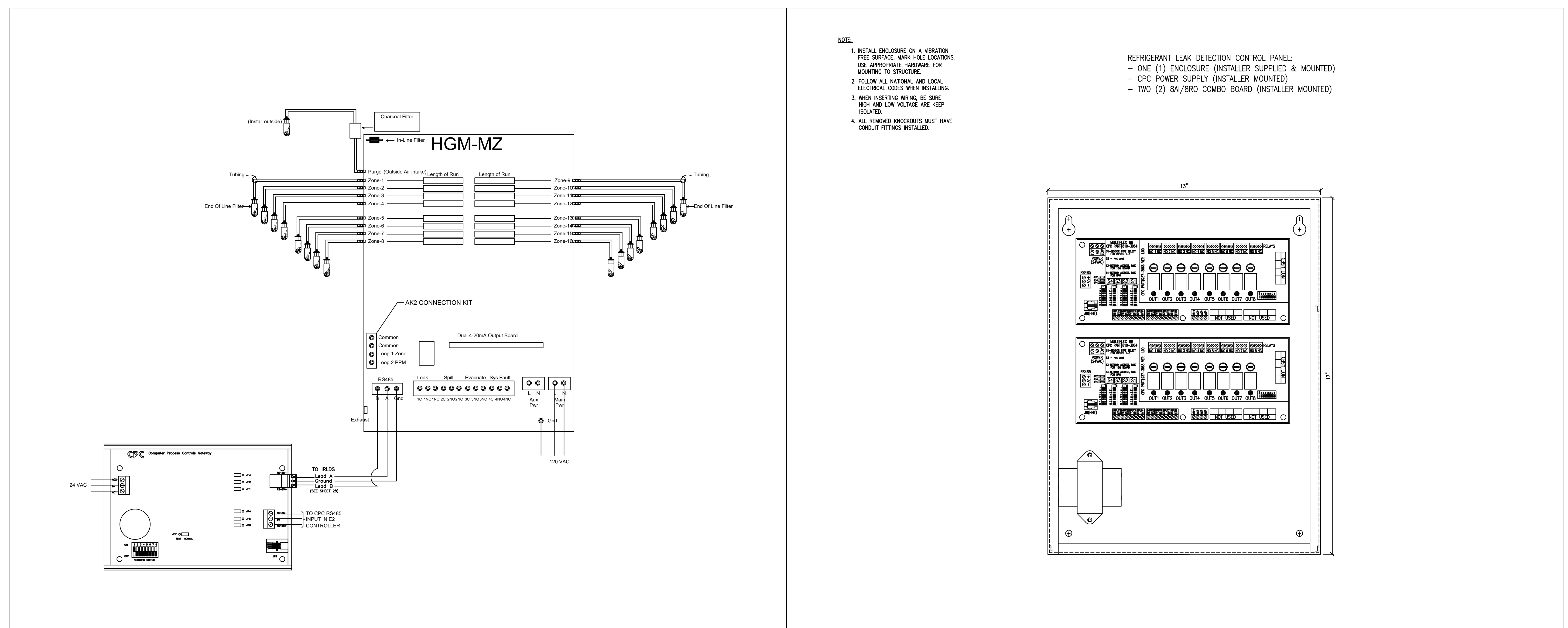
1 REFRIGERANT LEAK DETECTION UNIT - HGM MZ SCALE: NONE 2 CONTROL SYSTEM - DANFOSS LEAK DETECTION CONTROL PANEL SCALE: NONE
