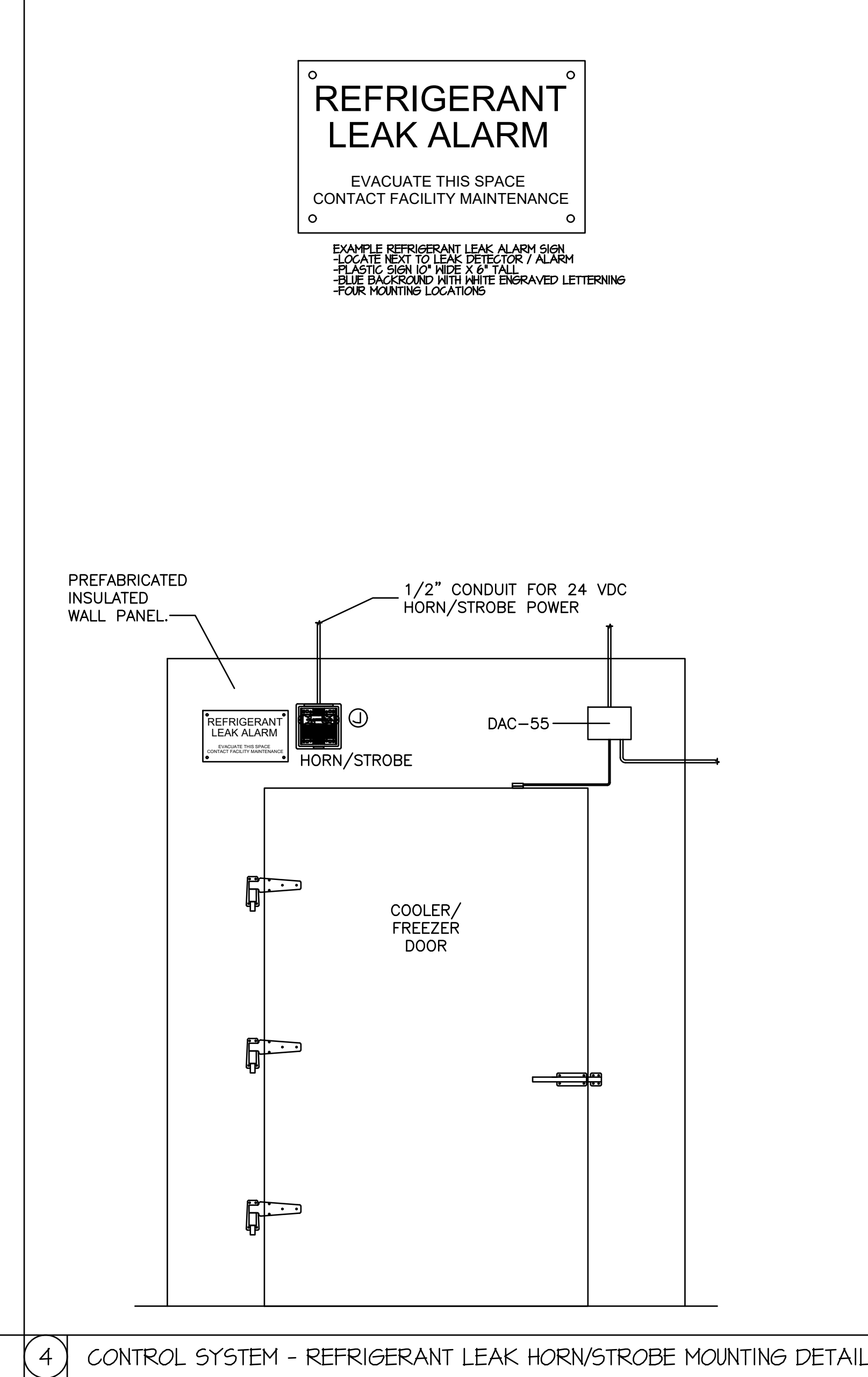
4 CONTROL SYSTEM - REFRIGERANT LEAK HORN/STROBE MOUNTING DETAIL
