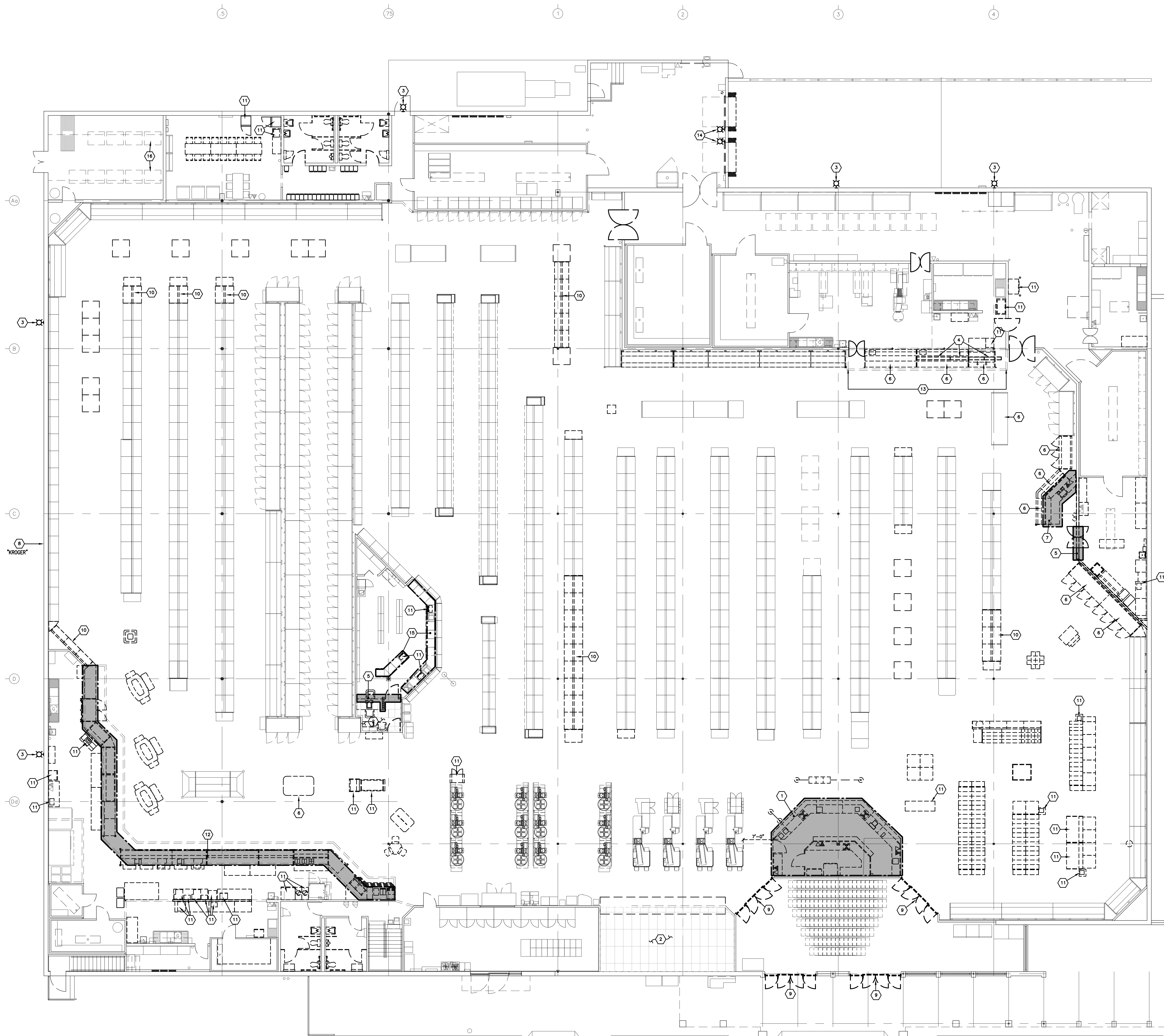
1 ELECTRICAL DEMOLITION PLAN ED1.1 3/32" = 1'-0"
